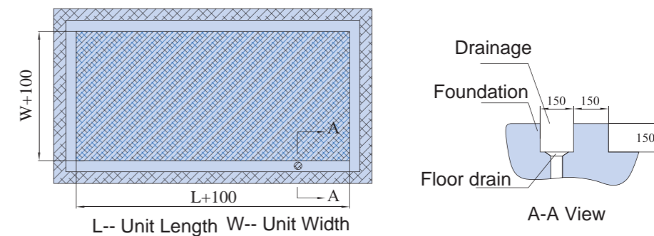
Foundation Diagram
